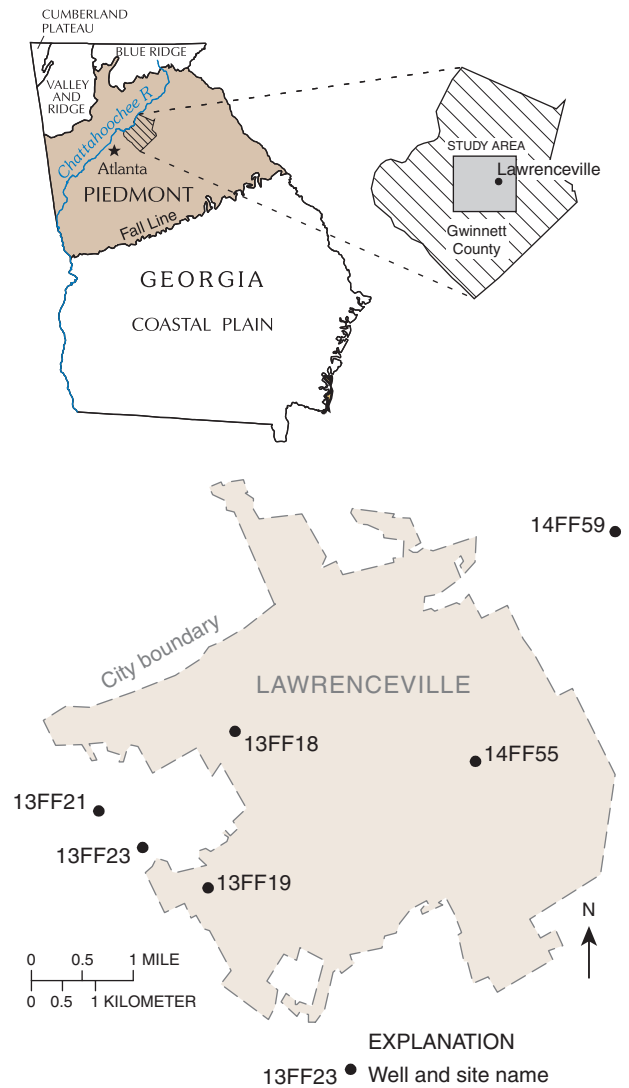
Figure 1. Study area and locations of wells sampled for chlorofluorocarbons, Lawrenceville, Georgia, 2001.
