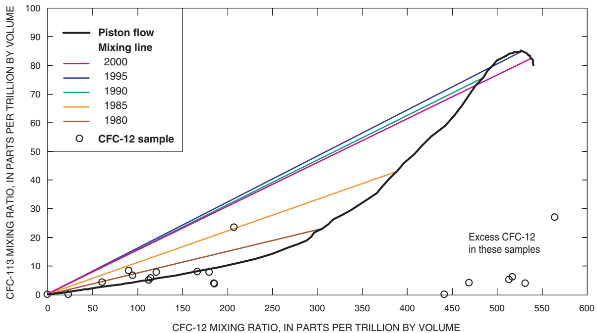
Figure 2. Mixing ratios of chlorofluorocarbon-113 (CFC-113) and chlorofluorocarbon-12 (CFC-12) for samples collected from six wells in Lawrenceville, Georgia, August–October 2001. The cluster of samples along the piston-flow line was obtained from two of the six wells sample. Other samples had excess CFC-12 and plot to the lower right or plot off the chart.
