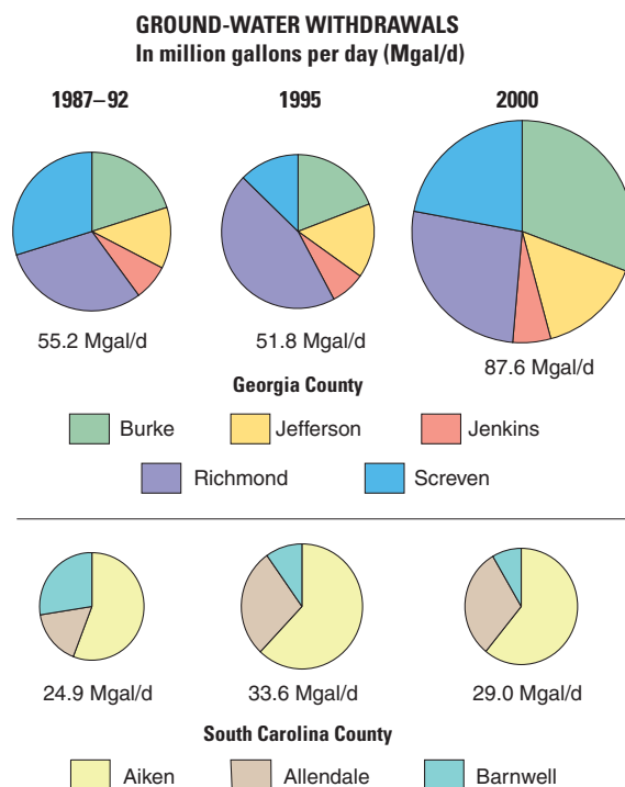
Figure 4. Ground-water use by county, Georgia and South Carolina, 1987–2000.
