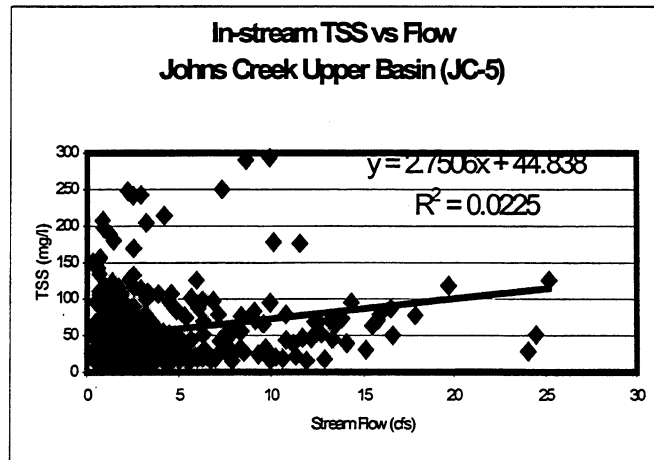
Figure 1. Correlations between in-stream levels of TSS in Johns Creek versus solids washoff or flow at each sampling station. Data were simulated results of BASINS model.
