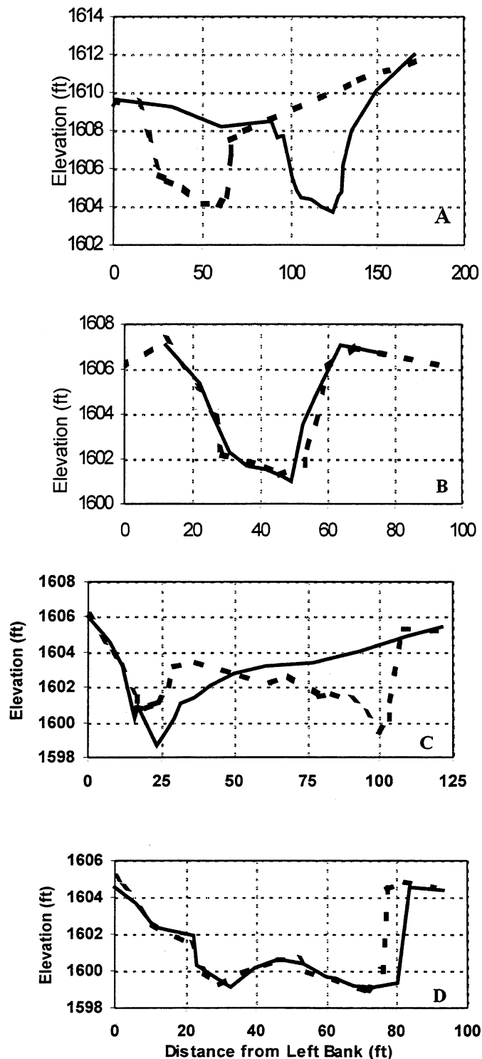
Figure 1. Left Fork Soque River Cross-Sections (Broken Line = Pre-Construction, April-June 1998, Solid Line = Post-Construction, Dec. 2000; A = LFS10, B = LFS50, C = LFS60, D = LFS70; Vertical Axis Exaggerated)
