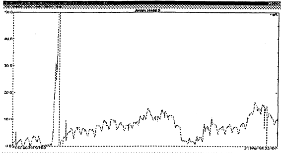
Figure 2. NH 4 -N (mg/L) Time Series In The Inner Channel Around The Time The Water Level Was Adjusted.
