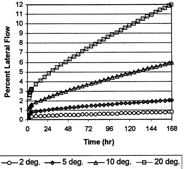
Figure 2. Percent of infiltration flowing laterally under four different slope conditions.
