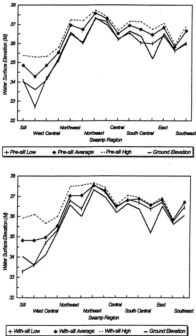
Figure 2. Pre-sill (top graph) and post-sill (bottom graph) water surface elevations across the Okefenokee Swamp, GA, during average, high, and low water conditions.
