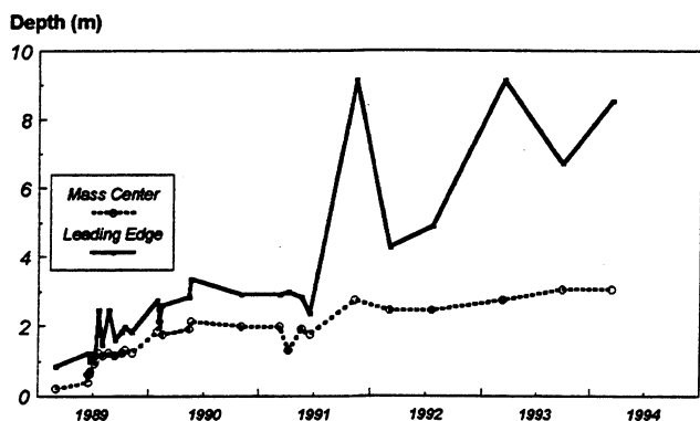
Figure 2. Observed center of mass and the leading edge of the plot mean Br - plume in the soil over time.
