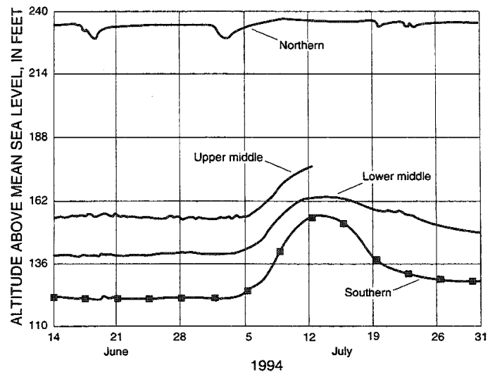
Figure 7. Water-level fluctuations in wells tapping the Upper Floridan aquifer, June 14-July 31, 1994.
