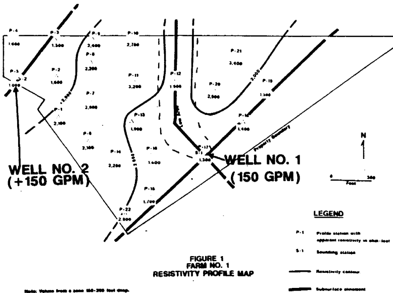
Figure 1. Resistivity Profile Map for Farm No. 1. (Note: Values from a zone 150-200 feet deep.)
