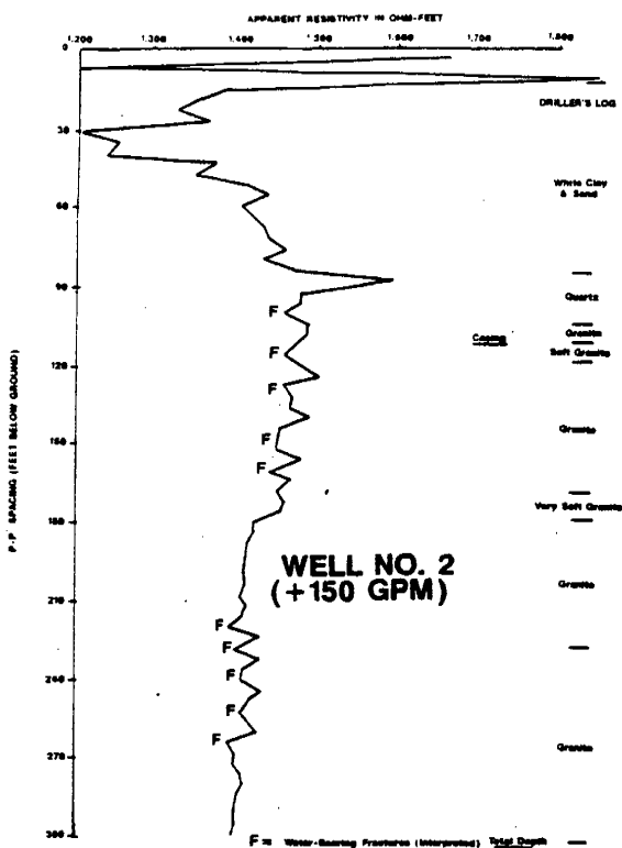
Figure 3. Sounding S-2 for Farm No. 1; Apparent resistivity in ohm-feet versus P-P' spacing in units of feet below ground. (F = Water-bearing fracture, as interpreted.)
