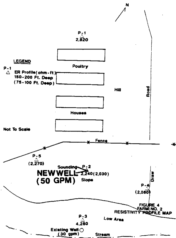
Figure 4. Resistivity Profile Map for Farm No. 2.
