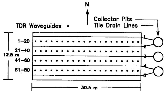
Figure 1. Diagram of plot 2 showing positions of 5 tile drain lines and 80 TDR installations. At each TDR location, waveguides 30, 60, and 90 cm in length were installed vertically.
