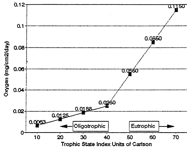
Figure 1. Conversion Scale for Hypolimnetic Oxygen Deficit and the Trophic State Index of Carlson.
