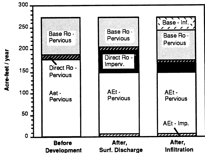
Figure 2. Predicted dispositions of water under alternative management scenarios in the main watershed of the Oconee County High School development site. (Ro, runoff; Imp., impervious; Inf., infiltration.)
