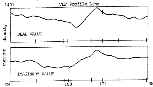
Figure 5. Current density along VLF profile line 1401.
