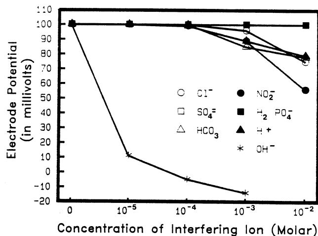
Figure 2. Effect of the Addition of Various Ions on \text{NO}_3 Selective Electrode Response in 10^{-3} M \text{NO}_3 -N
