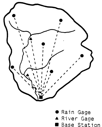
Figure 1. Example of ALERT Reporting Network
